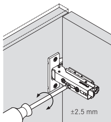
Height adjustment via base plate
