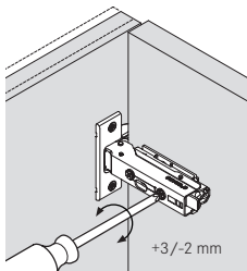
Depth adjustment via worm gear
